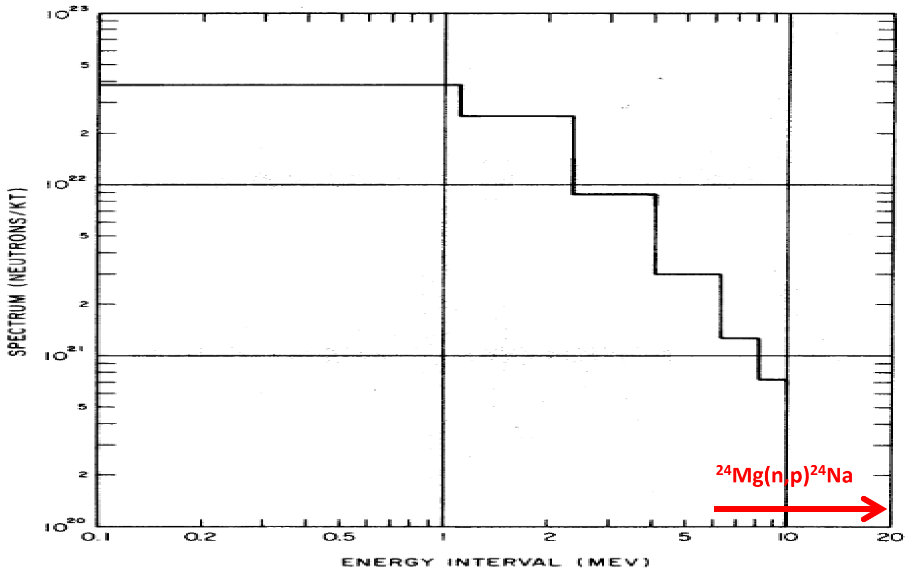
Figure 8.116a. Neutron spectrum for a fission weapon per kiloton total energy yield.
