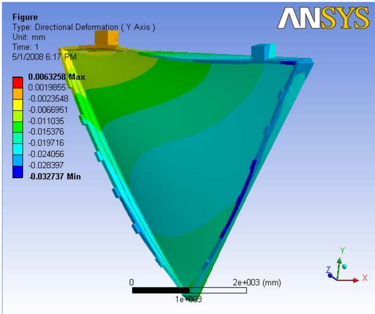
FIGURE 13 Ideal slice with Gravity, Hexcel (No Rods, No wire loads) > Static Structural > Solution > Z - Directional Deformation > Figure
