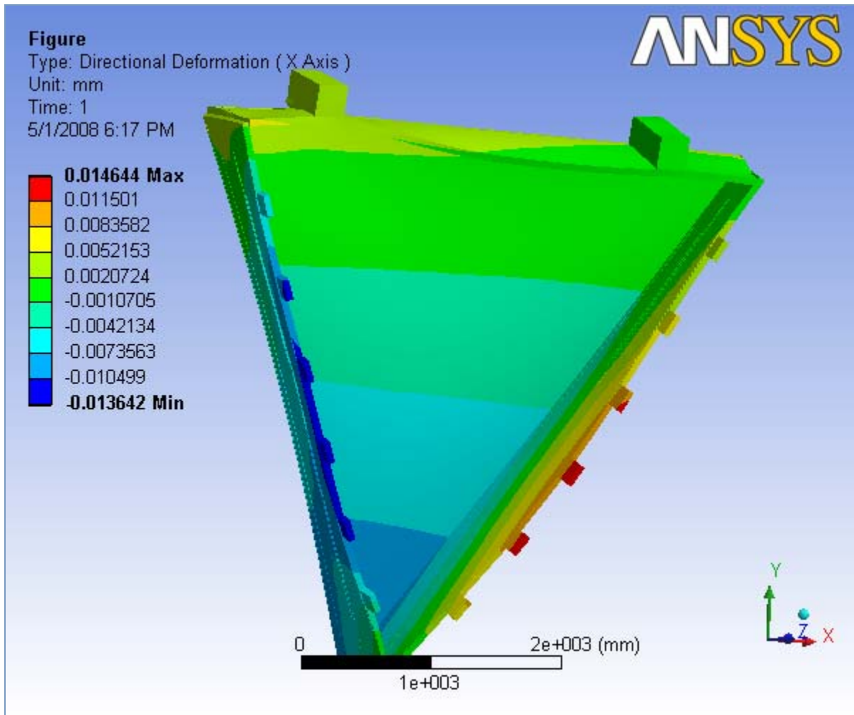
FIGURE 12 Ideal slice with Gravity, Hexcel (No Rods, No wire loads) > Static Structural > Solution > Y - Directional Deformation > Figure
