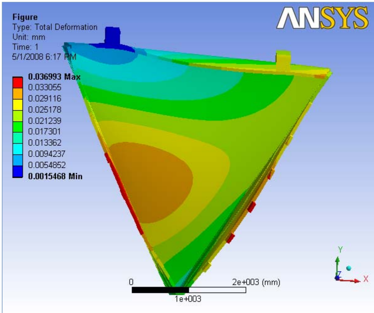
FIGURE 11 Ideal slice with Gravity, Hexcel (No Rods, No wire loads) > Static Structural > Solution > X - Directional Deformation > Figure
