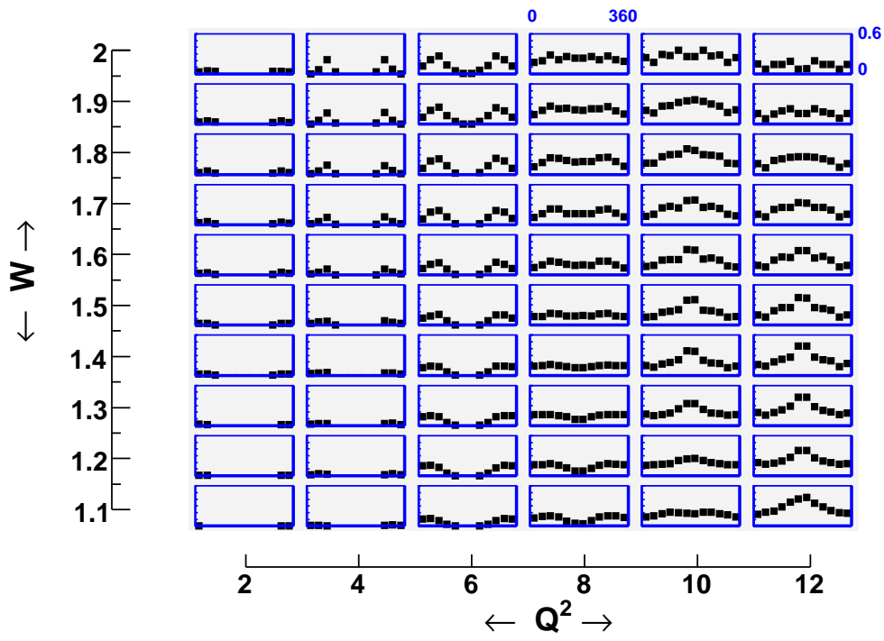
Figure 36: \phi_\pi evolution of the \pi^0 acceptance in the forward \cos\theta_\pi = 0.1 \pm 0.1 bin for the resonance region and the proposed Q^2 range.
