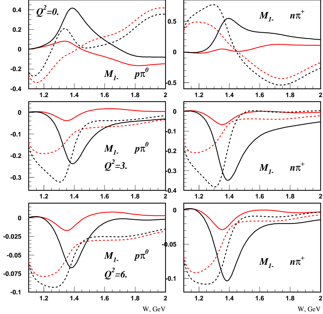
Figure 10: The M_{1-} multipole amplitude for the reactions \gamma^*p \rightarrow p\pi^0 (left) and n\pi^+ (right) at Q^2 = 0, 3, \text{ and } 6 (GeV/c)^2 . Black curves are the total amplitudes, red curves represent the background; each separated into imaginary (real) part and represented by solid (dashed) curves.
