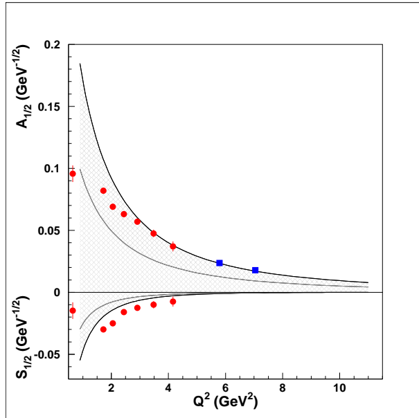
Figure 2: Transition N - N^*(1535) amplitudes based on LCSR, that utilized preliminary LQCD results of Distribution Amplitudes [55] in comparison with the data. CLAS data [109] are shown in red, while preliminary data on (A_{1/2}^2 + \epsilon S_{1/2}^2)^{1/2} combination of transition amplitudes at high Q^2 are shown in blue.
