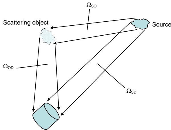
Figure 19: Determination of the flux efficacy factor for neutron-scattering objects in the environment.
