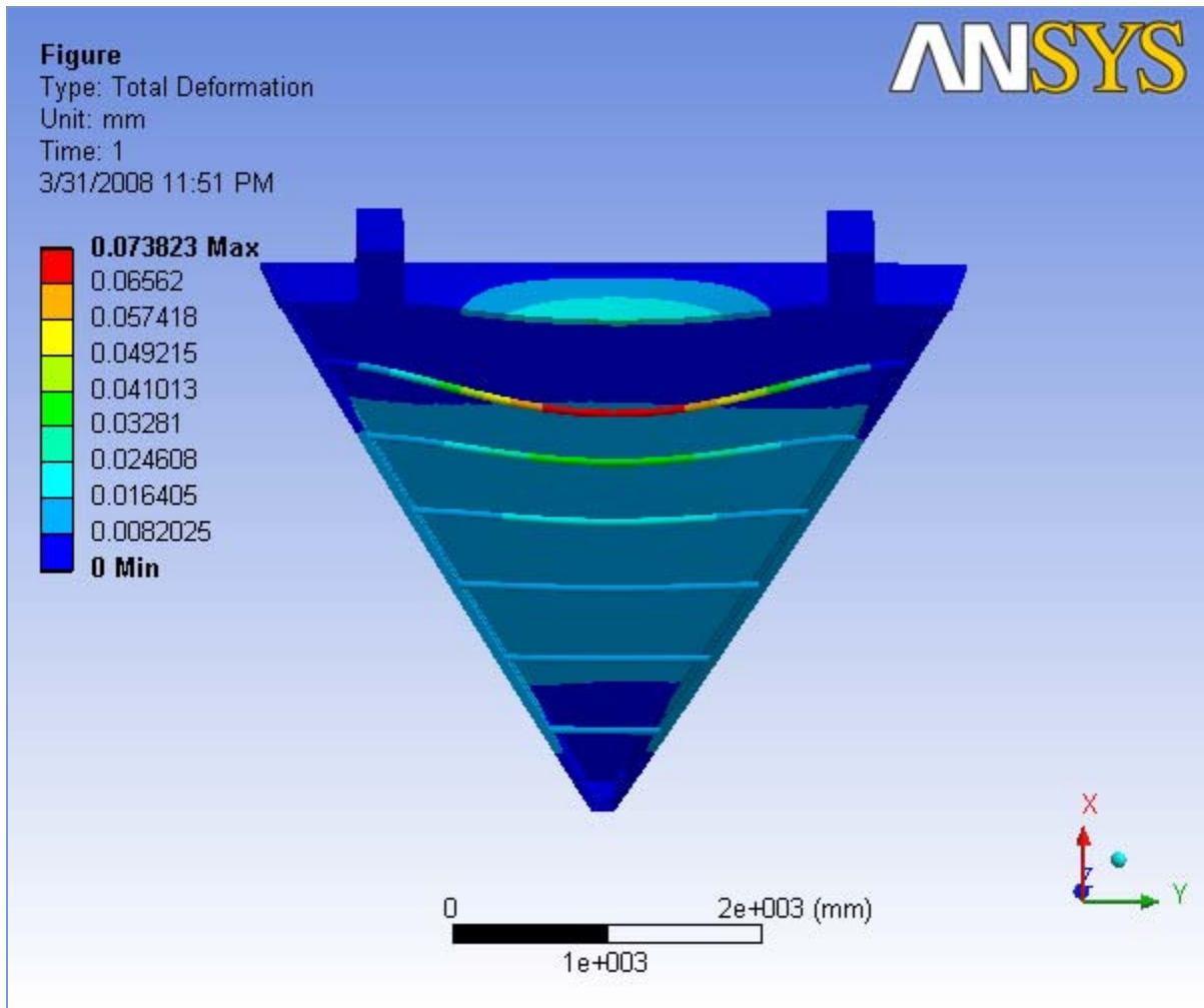
FIGURE 9 Analysis 6.2 > Static Structural > Solution > x Directional Deformation > Figure
