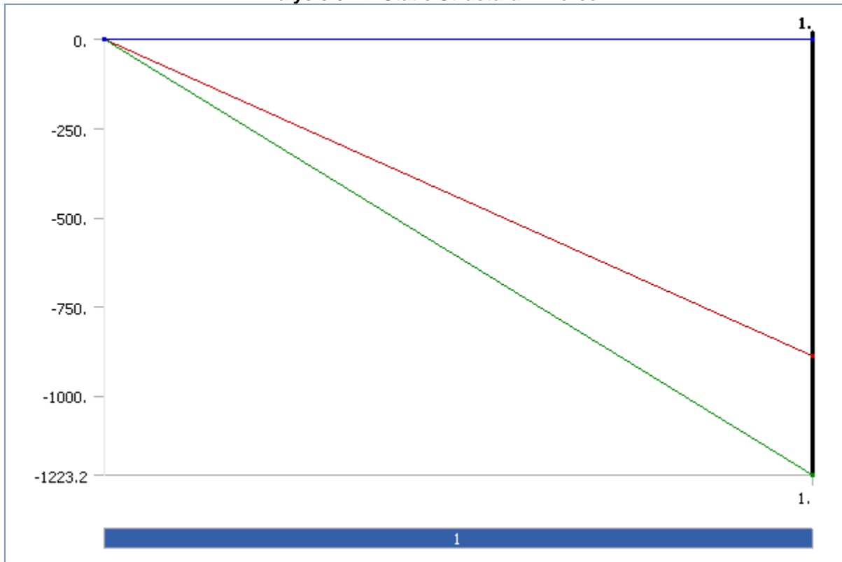
FIGURE 4 Analysis 6.2 > Static Structural > Force
