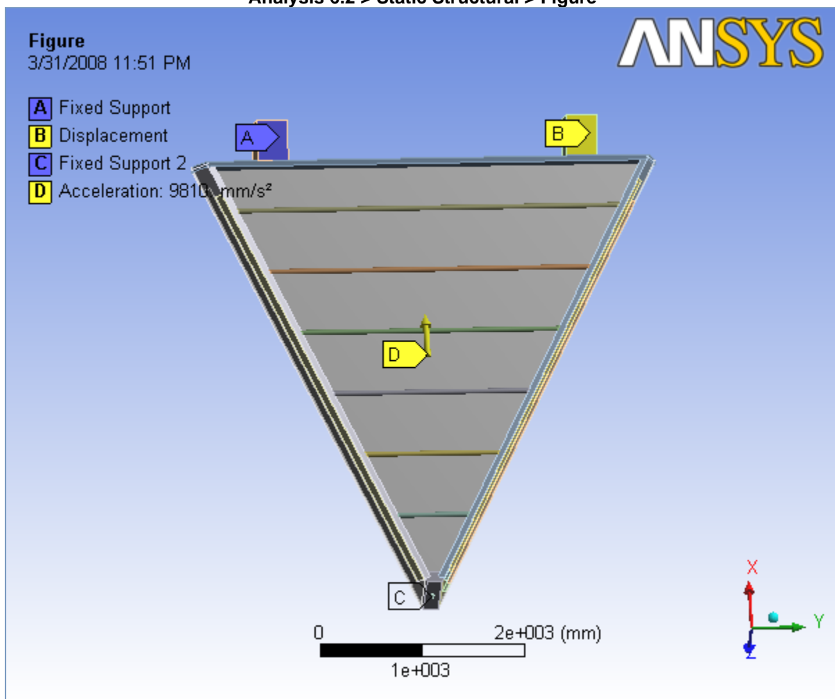
FIGURE 1 Analysis 6.2 > Static Structural > Figure
