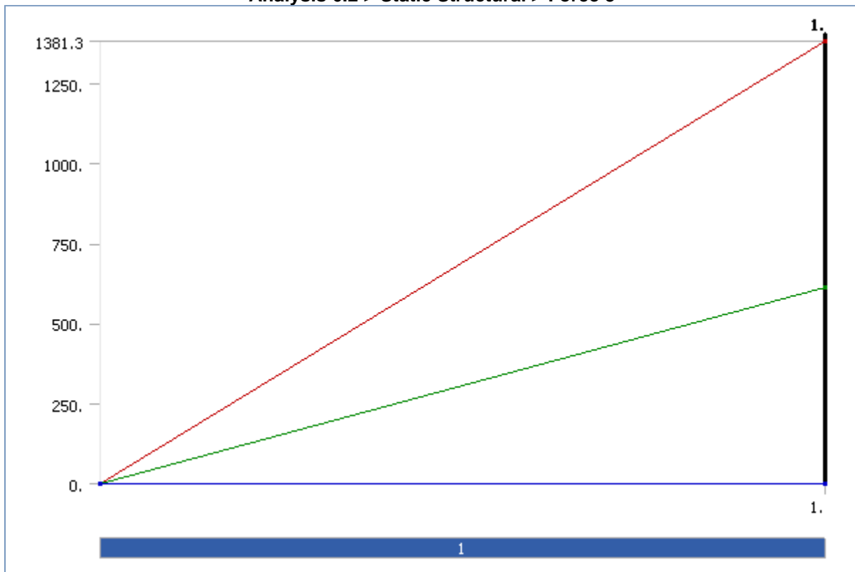
FIGURE 6 Analysis 6.2 > Static Structural > Force 3
