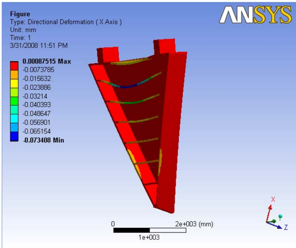
FIGURE 10 Analysis 6.2 > Static Structural > Solution > y Directional Deformation > Figure
