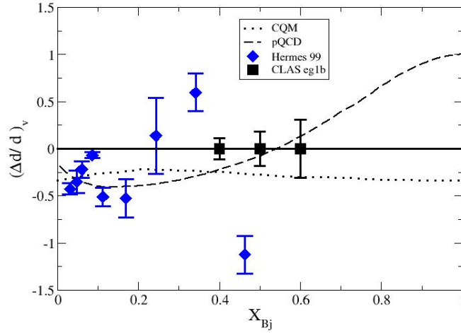
Figure 9. The ratio of polarized to unpolarized valence down quark distribution function vs x_{Bj} [21] .
