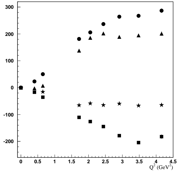
Figure 16: The A_{1/2}(Q^2) helicity amplitudes are scaled by Q^3/1.0 \text{ GeV}^2 and shown for the Roper P_{11}(1440) (triangles), S_{11}(1535) (circles), D_{13}(1520) (squares), and F_{15}(1680) (stars). At the highest currently accessible momentum transfers the Q^2 dependence is consistent with a flat behavior.
