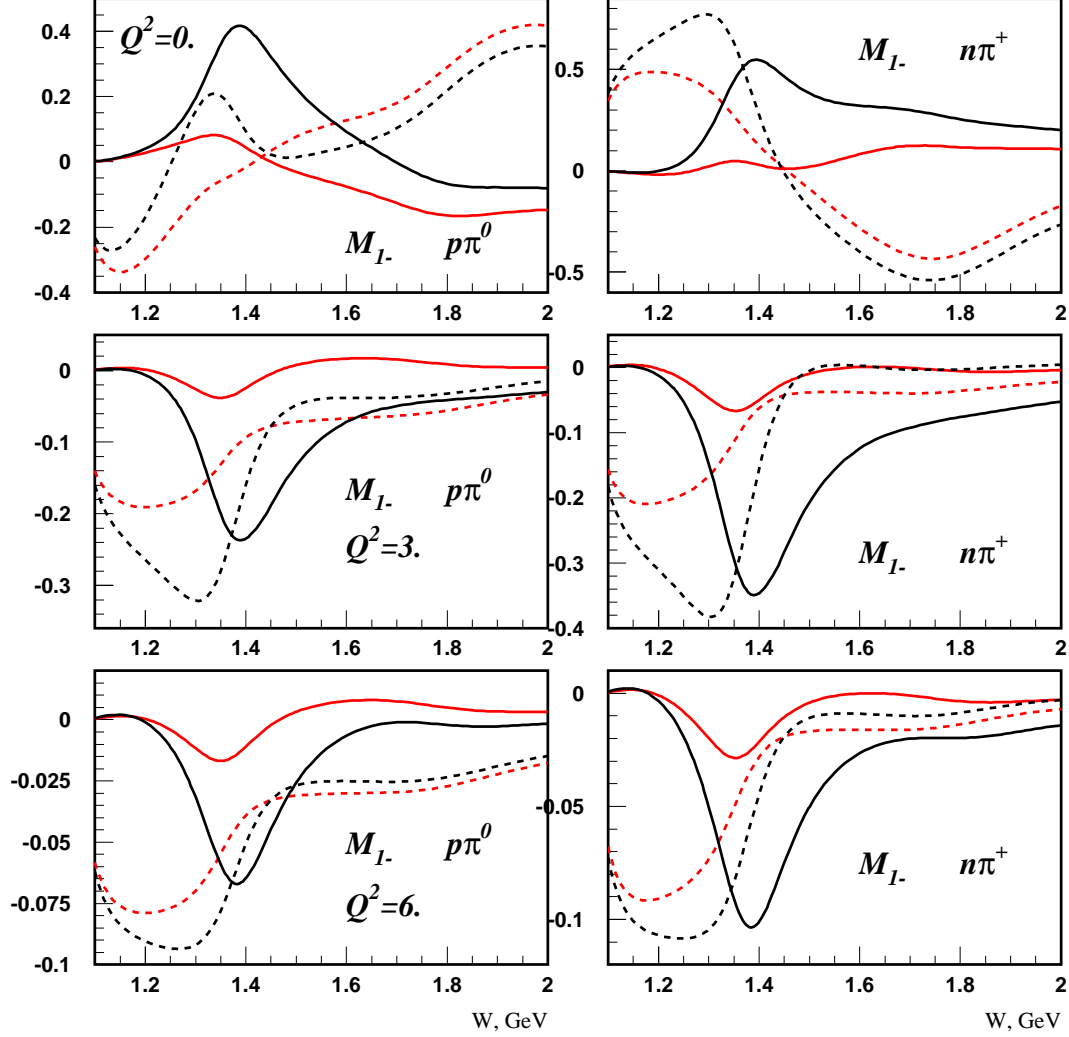
Figure 10: The M_{1-} multipole amplitude for the reactions \gamma^*p \rightarrow p\pi^0 (left) and n\pi^+ (right) at Q^2 = 0, 3, and 6 \text{ GeV}^2 . Black curves are the total amplitudes, red curves represent the background; each separated into imaginary (real) part and represented by solid (dashed) curves.
