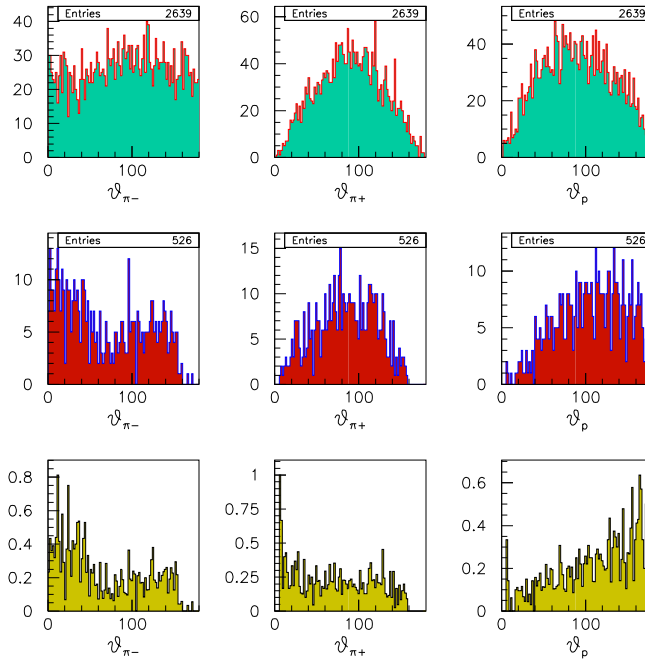
Figure 24: Efficiency for various angular distributions in 2\pi production averaged over the four other kinematics variables at W from 1.5 to 1.7 GeV and at Q^2 from 5.0 to 10.0 \text{GeV}^2 . The distributions for generated and accepted events are shown in the top and middle row, respectively. The estimated efficiencies are presented in the bottom row.
