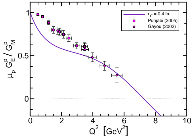
Figure 4: Ratio \mu_p G_E^p/G_M^p(Q^2) of the proton form factor. The solid curve is calculated from the covariant model based on the Dyson-Schwinger equation [72].
