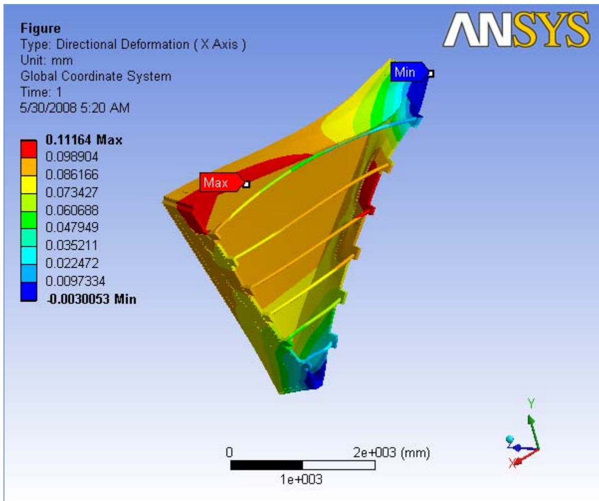
FIGURE 12 sector 1, Case 3 > Static Structural > Solution > Y - Directional Deformation > Figure
